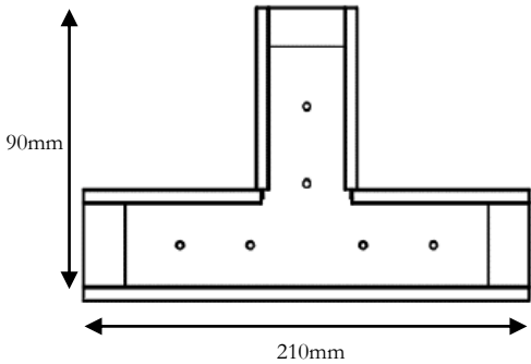
T connector SD-574
