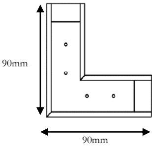
Horizontal connector SD-573
